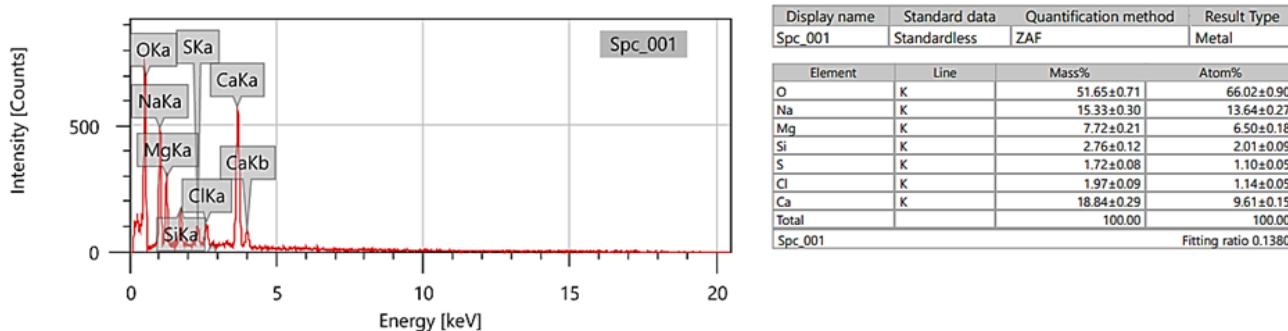
Fig. 4. EDX test results for the most (a) and least (b) polluted water samples collected from the area of study
