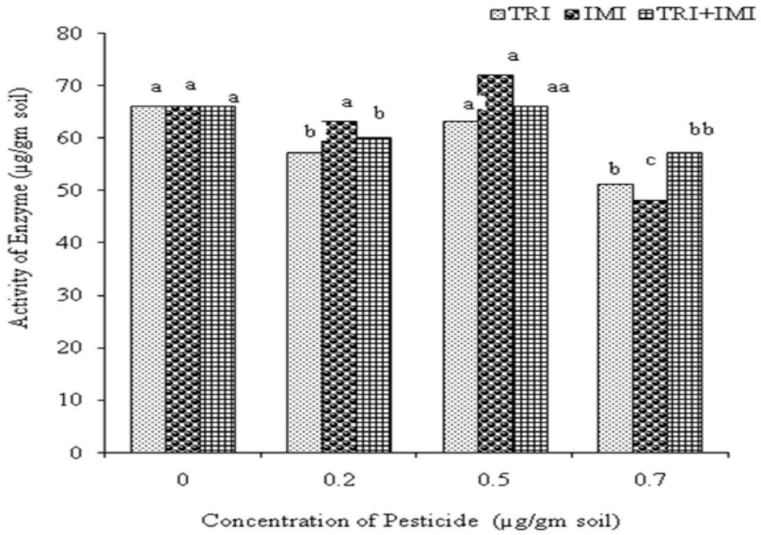
Fig. 2. Showing protease activity. TRI-Triadimefon, IMI-Imidacloprid, TRI+IMI-Triadimefon+Imidacloprid. Bars marked by the same letter are not significantly different ( P < 0.05 ) from each other according to DMR (Duncan's multiple range) test.
