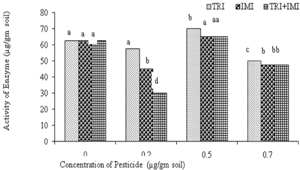
Fig.3. Showing urease activity. TRI-Triadimefon, IMI-Imidacloprid, TRI+IMI-Triadimefon+Imidacloprid. Bars marked by the same letter are not significantly different ( P < 0.05 ) from each other according to DMR (Duncan's multiple range) test.
