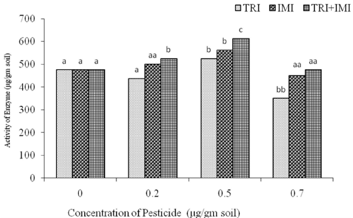
Fig.1. Showing the phosphatase enzyme activity. TRI-Triadimefon, IMI-Imidacloprid, TRI+IMI-Triadimefon+Imidacloprid. Bars marked by the same letter are not significantly different ( P < 0.05 ) from each other according to DMR (Duncan's multiple range) test.
